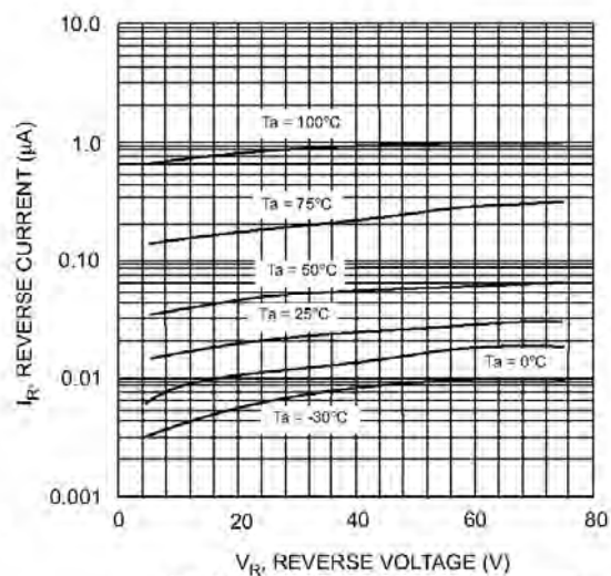
Fig. 2 Reverse Current vs Reverse Voltage
